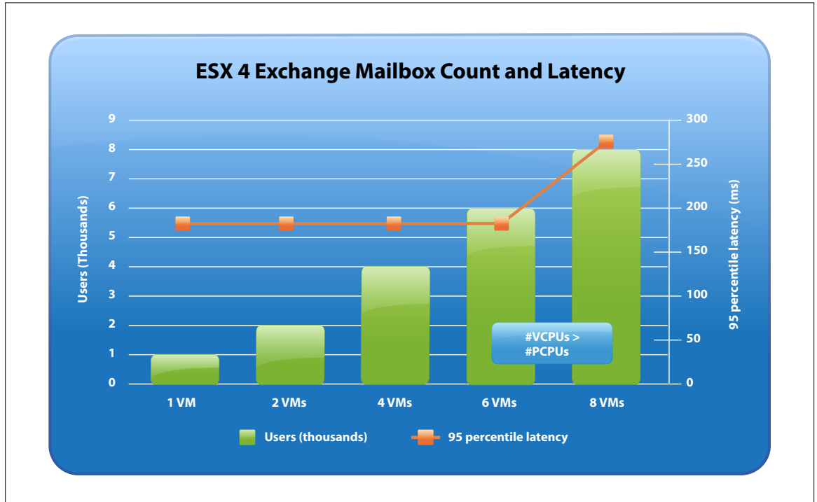
Figure 12 – vSphere performance enhancements with Microsoft Exchange
