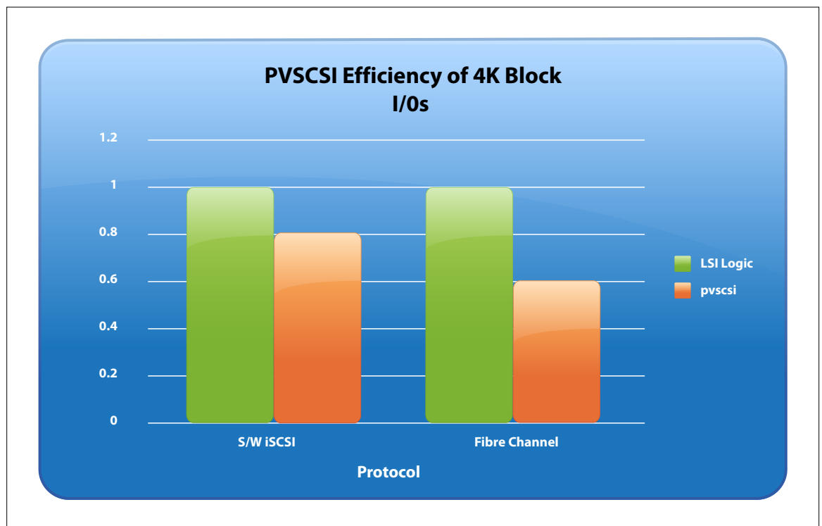
Figure 2 – Efficiency gains with PV SCSI adapter
