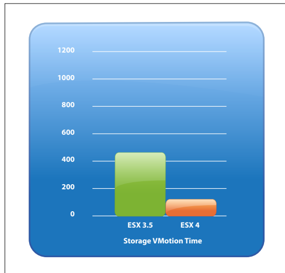
Figure 5 - Decreased Storage VMotion Time
