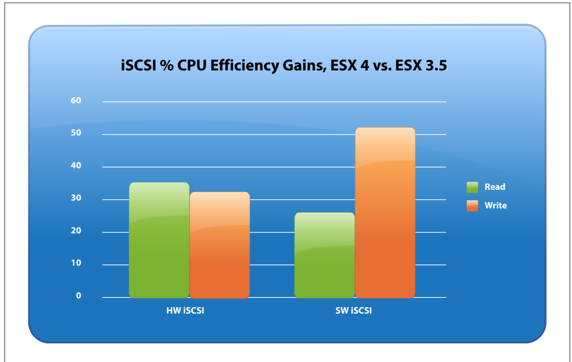
Figure 3 - iSCSI% CPU Efficiency Gains, ESX 4 vs. ESX 3.5
