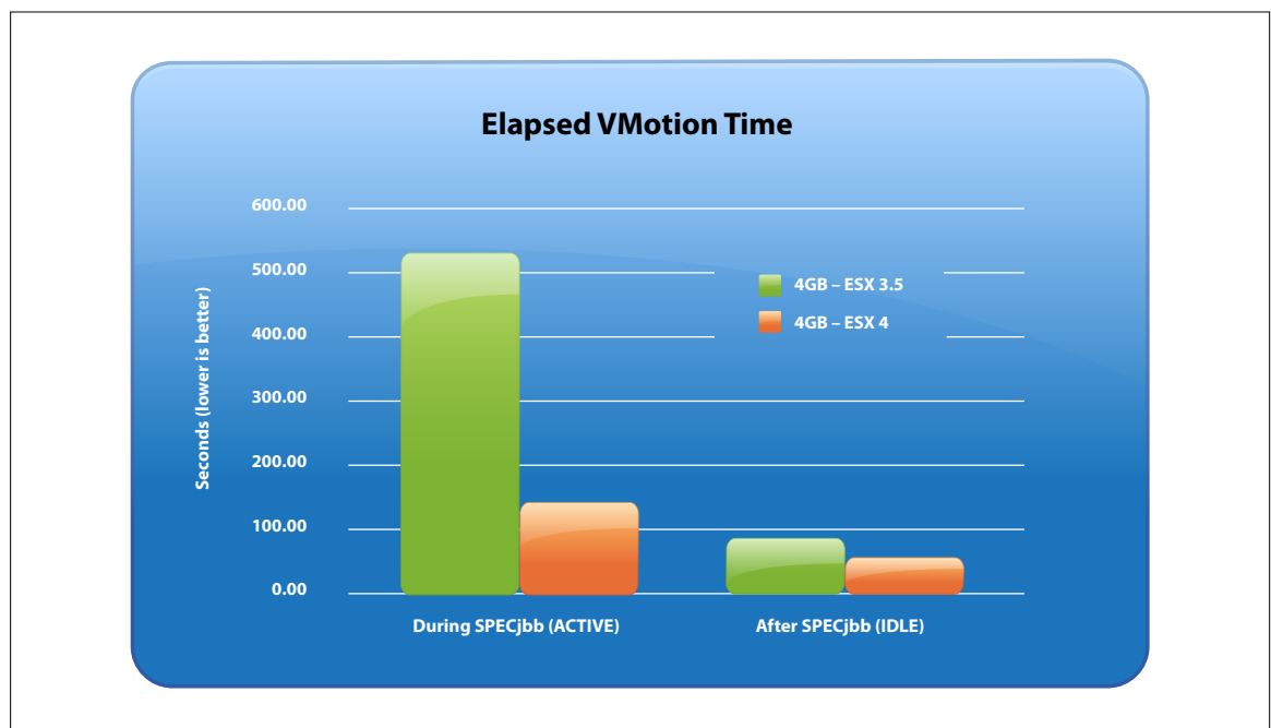
Figure 7 - Performance Enhancements Lead to a Reduced Time to VMotion
