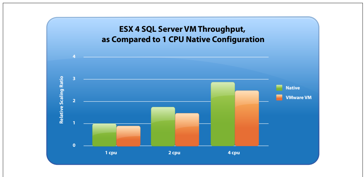
Figure 10 – Comparison of vSphere 4 SQL Server VM Throughput vs. Native Configuration
