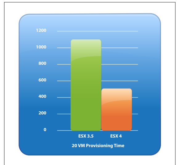
Figure 6 - Improved VMFS Performance
