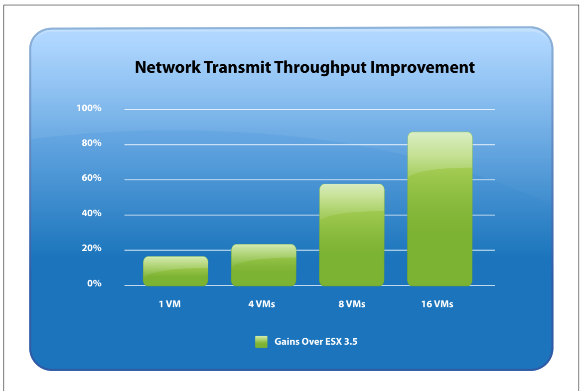
Figure 4 - Network Transmit Throughput Improvement for vSphere 4
