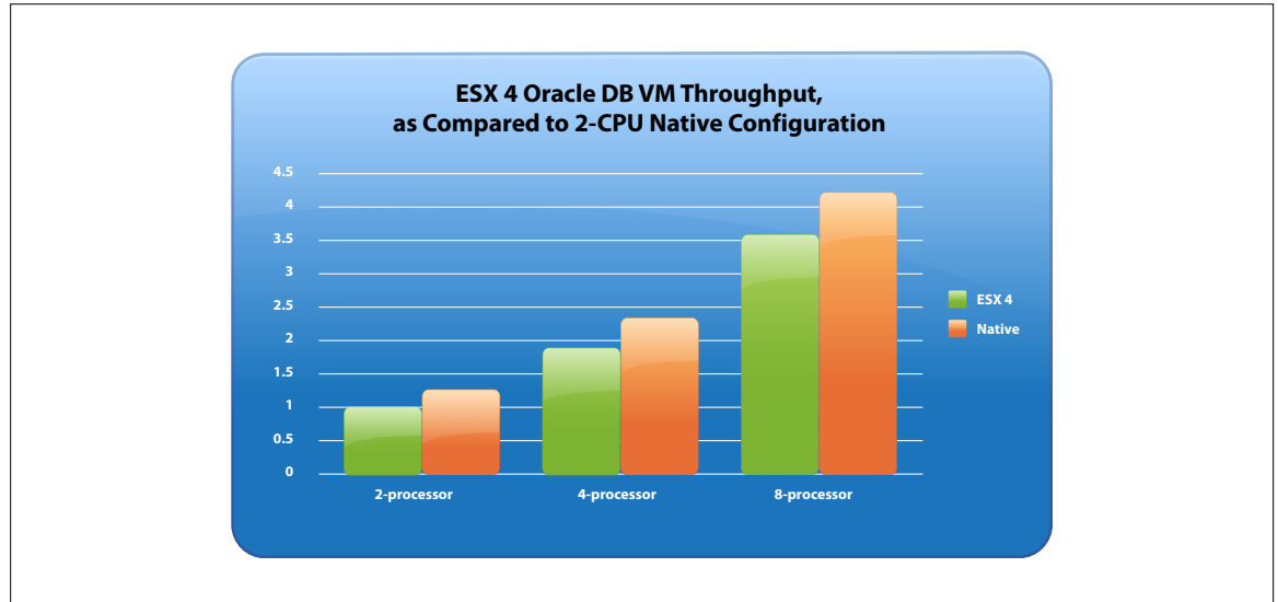
Figure 9 – Comparison of Oracle DB VM Throughput vs. 2-CPU Native Configuration
